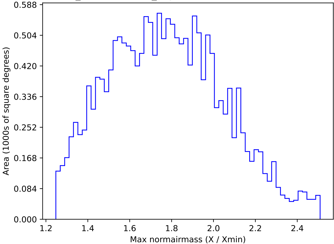
weather_cloudso30v3.4_10yrs WFD u band: Max normairmass
