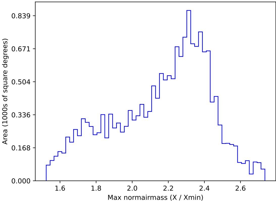
weather_cloudso30v3.4_10yrs WFD r band: Max normairmass
