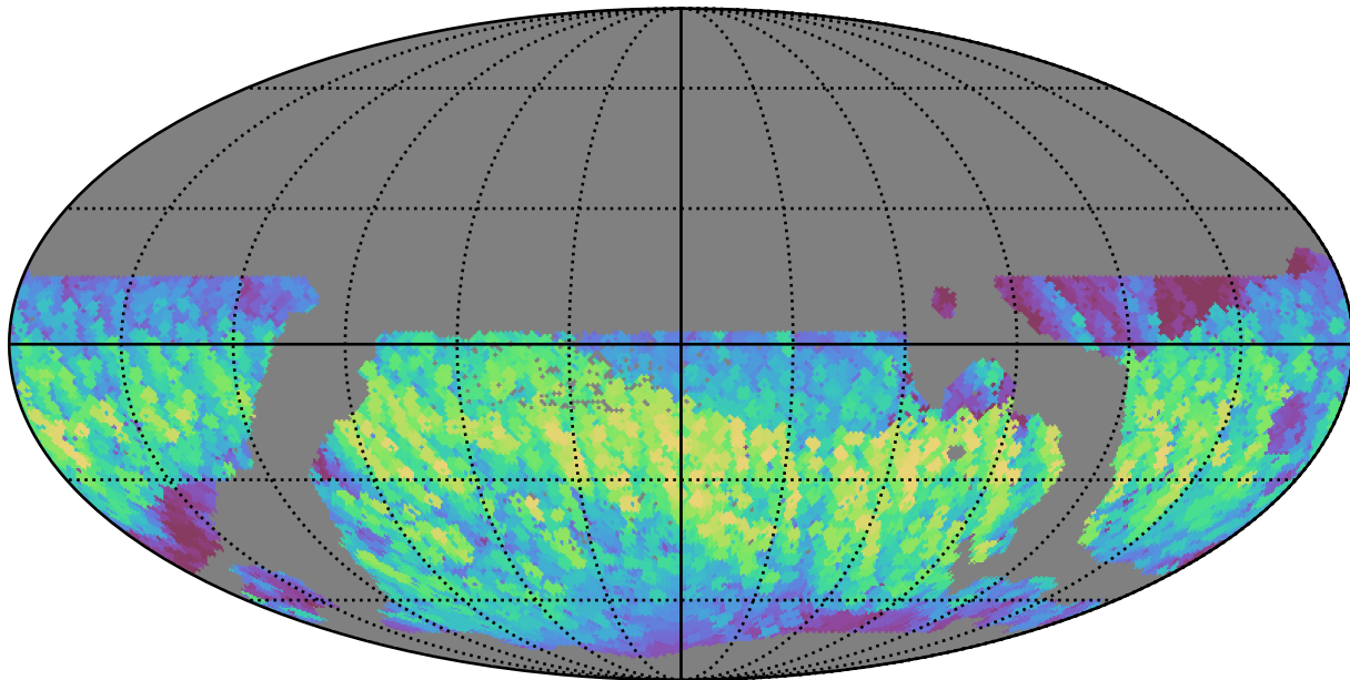
weather_cloudso30v3.4_10yrs WFD i band: Max normairmass
