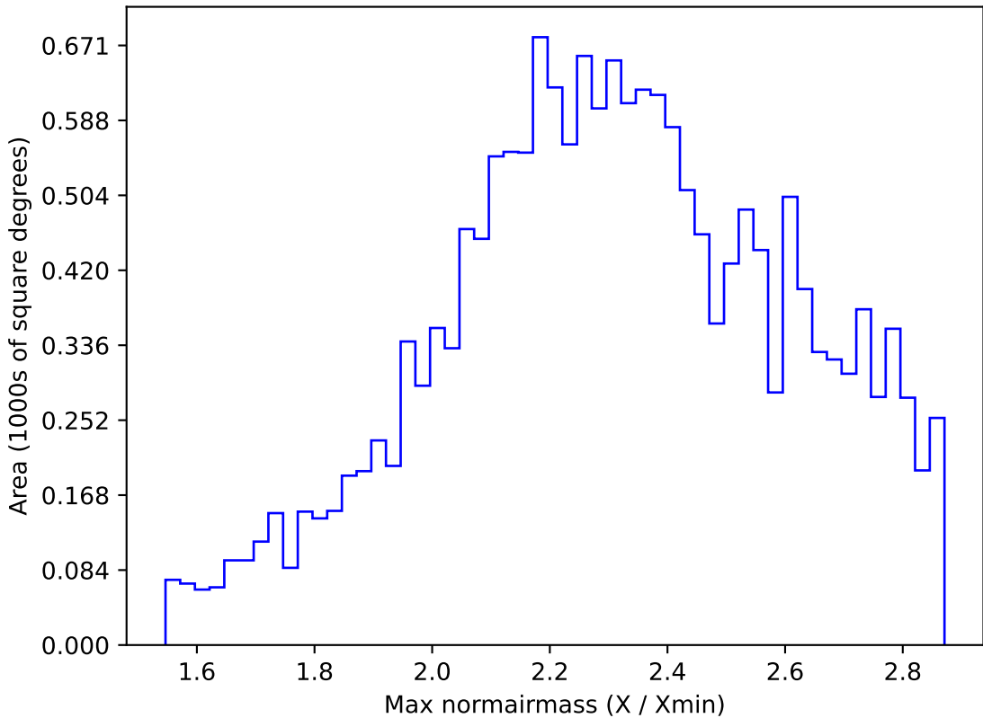
weather_cloudso30v3.4_10yrs WFD i band: Max normairmass
