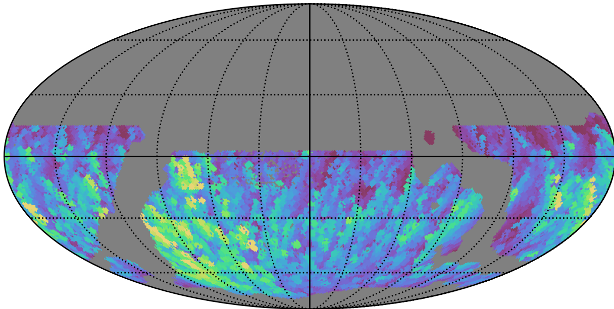
weather_cloudso30v3.4_10yrs WFD g band: Max normairmass
