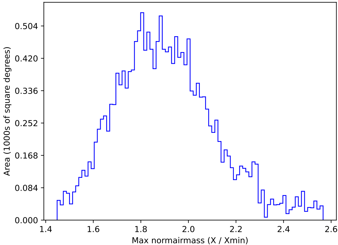
weather_cloudso30v3.4_10yrs WFD g band: Max normairmass
