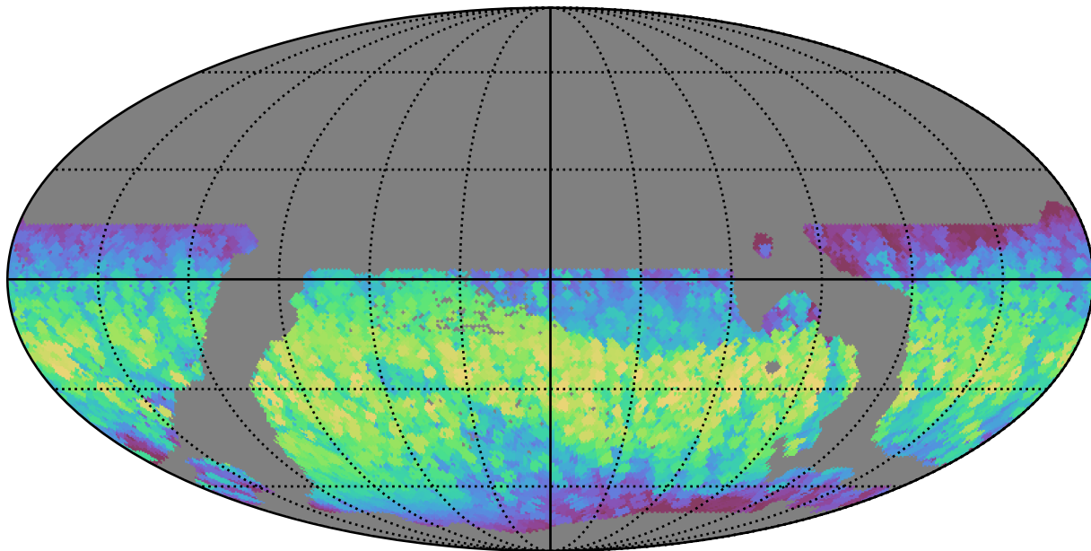
weather_cloudso30v3.4_10yrs WFD all bands: Max normairmass
