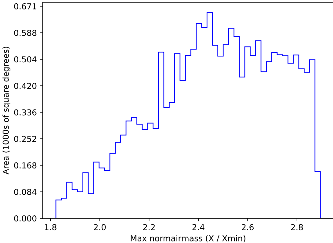
weather_cloudso30v3.4_10yrs WFD all bands: Max normairmass
