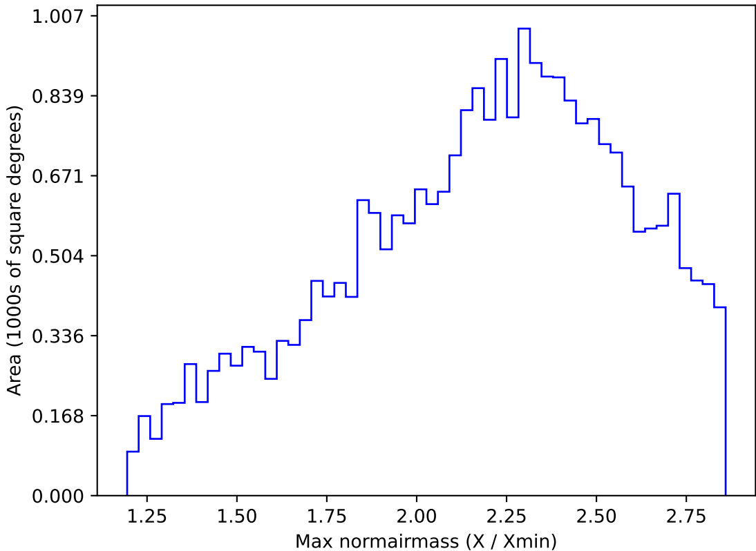
weather_cloudso30v3.4_10yrs All sky z band: Max normairmass
