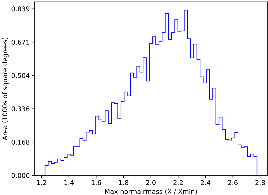
weather_cloudso30v3.4_10yrs All sky y band: Max normairmass
