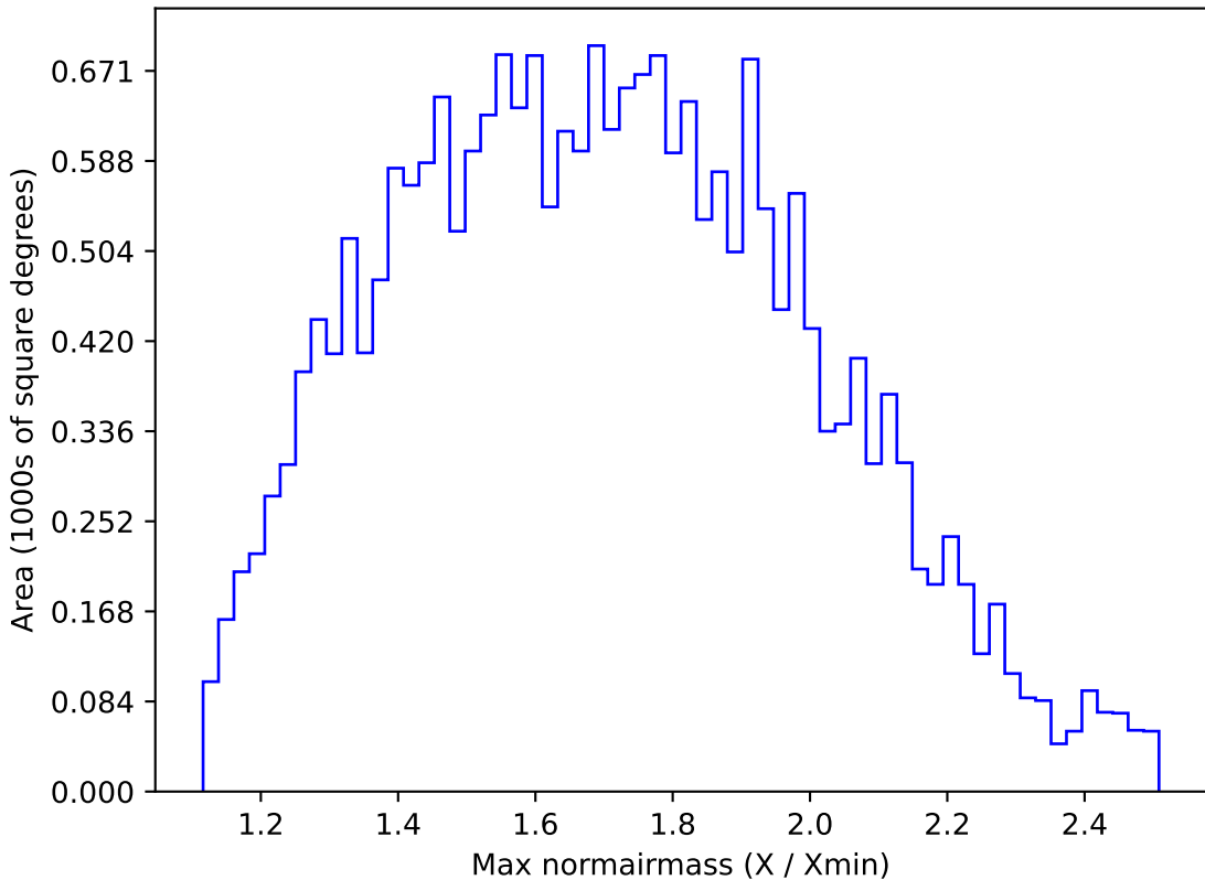
weather_cloudso30v3.4_10yrs All sky u band: Max normairmass
