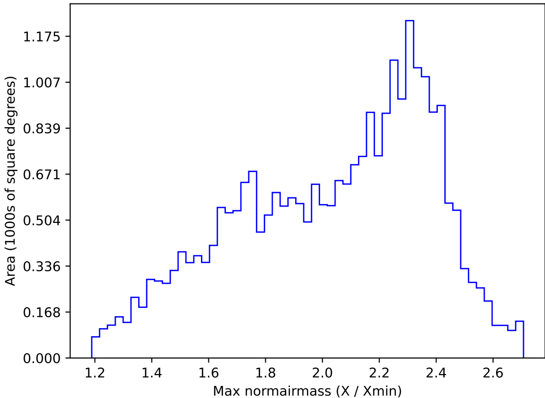
weather_cloudso30v3.4_10yrs All sky r band: Max normairmass
