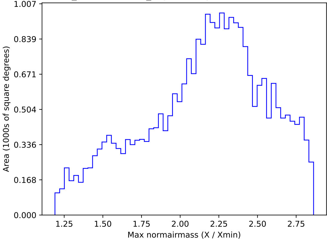
weather_cloudso30v3.4_10yrs All sky i band: Max normairmass
