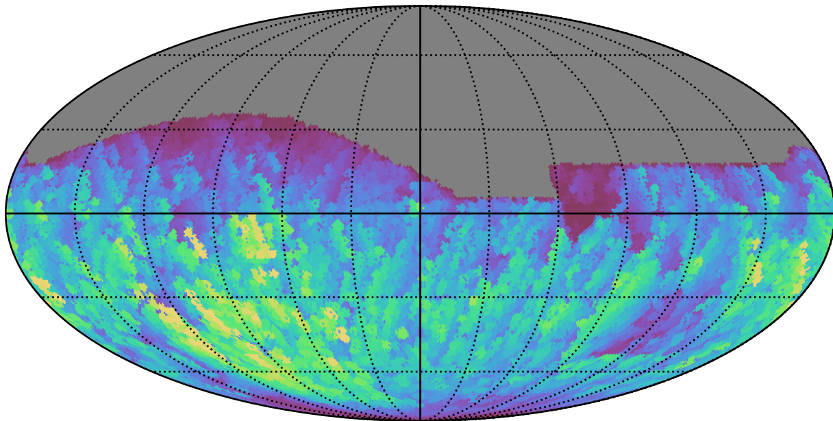
weather_cloudso30v3.4_10yrs All sky g band: Max normairmass
