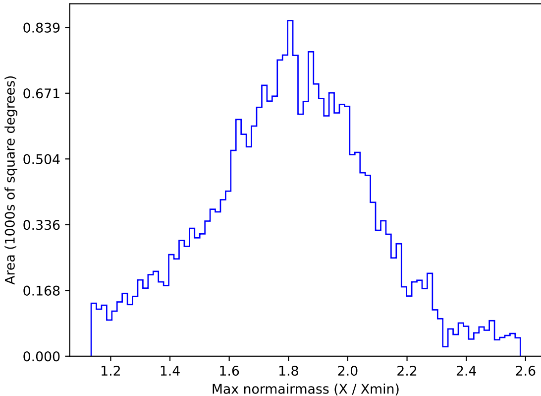
weather_cloudso30v3.4_10yrs All sky g band: Max normairmass
