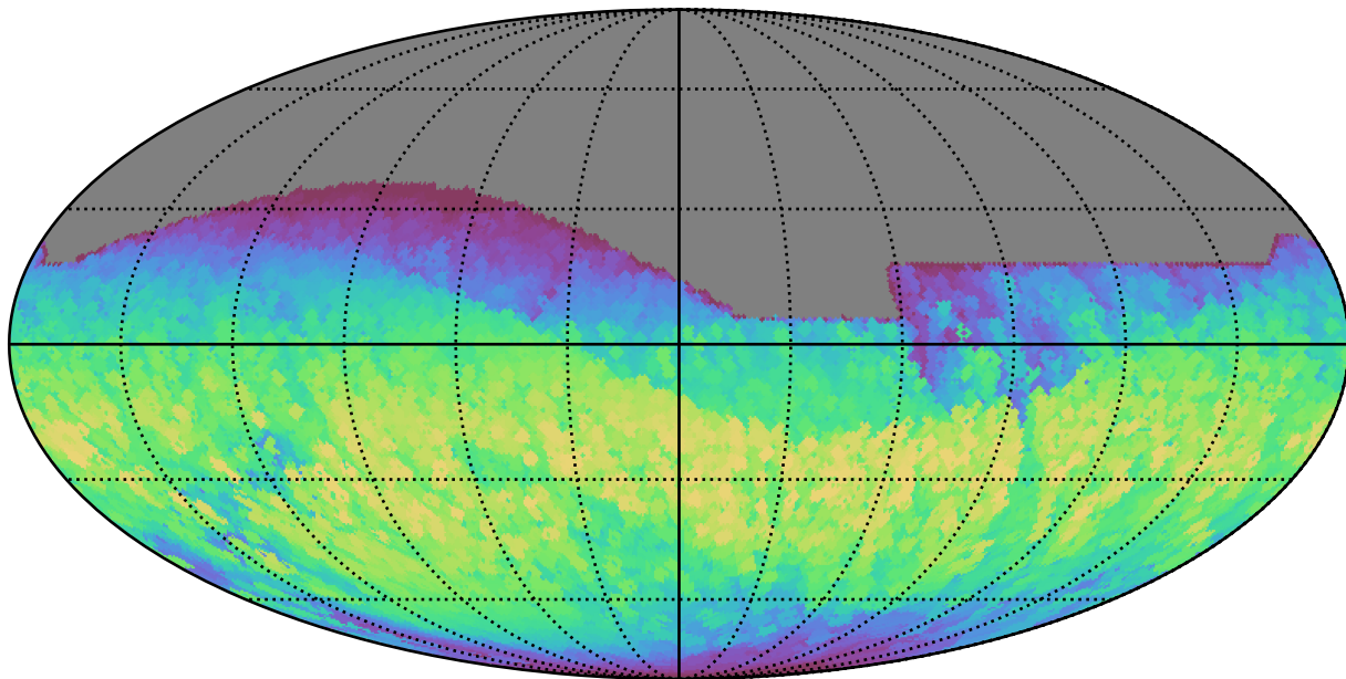
weather_cloudso30v3.4_10yrs All sky all bands: Max normairmass
