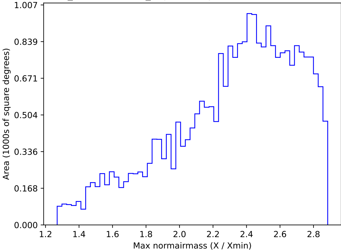
weather_cloudso30v3.4_10yrs All sky all bands: Max normairmass
