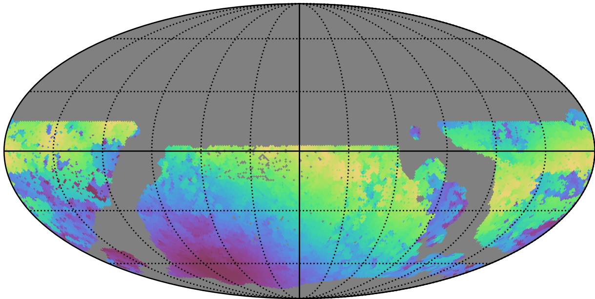
weather_cloudso30v3.4_10yrs WFD y band: Max moonDistance
