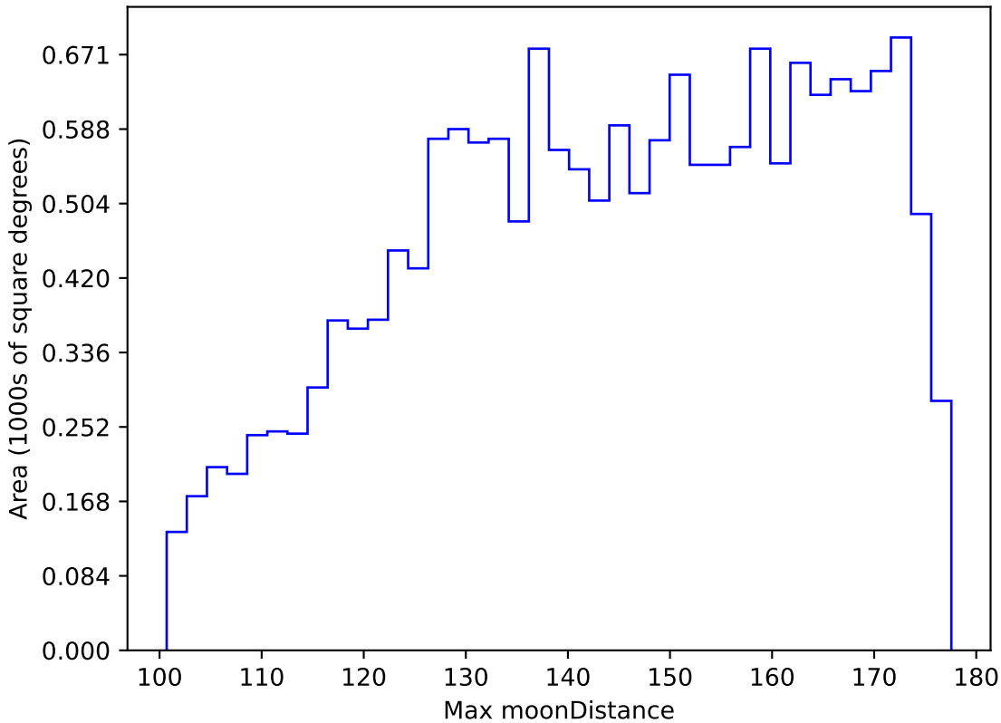
weather_cloudso30v3.4_10yrs WFD y band: Max moonDistance
