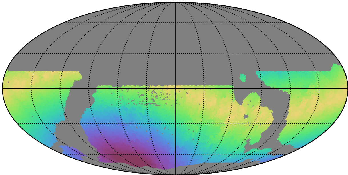
weather_cloudso30v3.4_10yrs WFD u band: Max moonDistance
