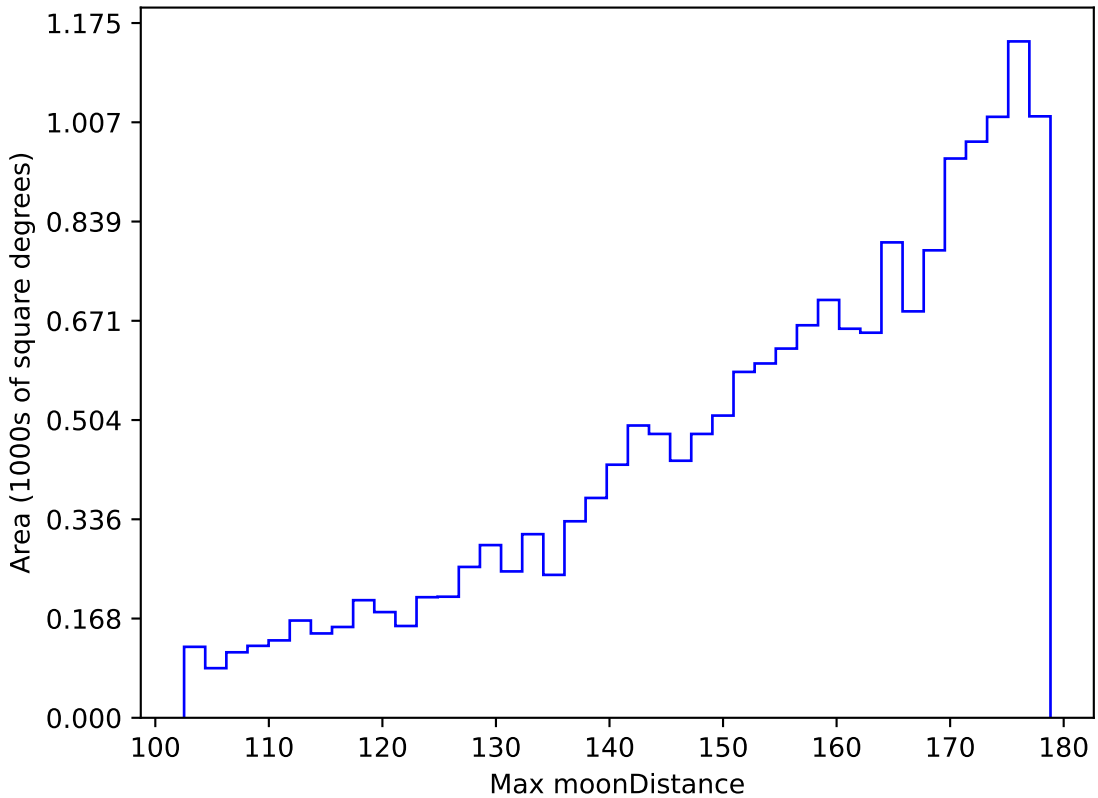
weather_cloudso30v3.4_10yrs WFD u band: Max moonDistance
