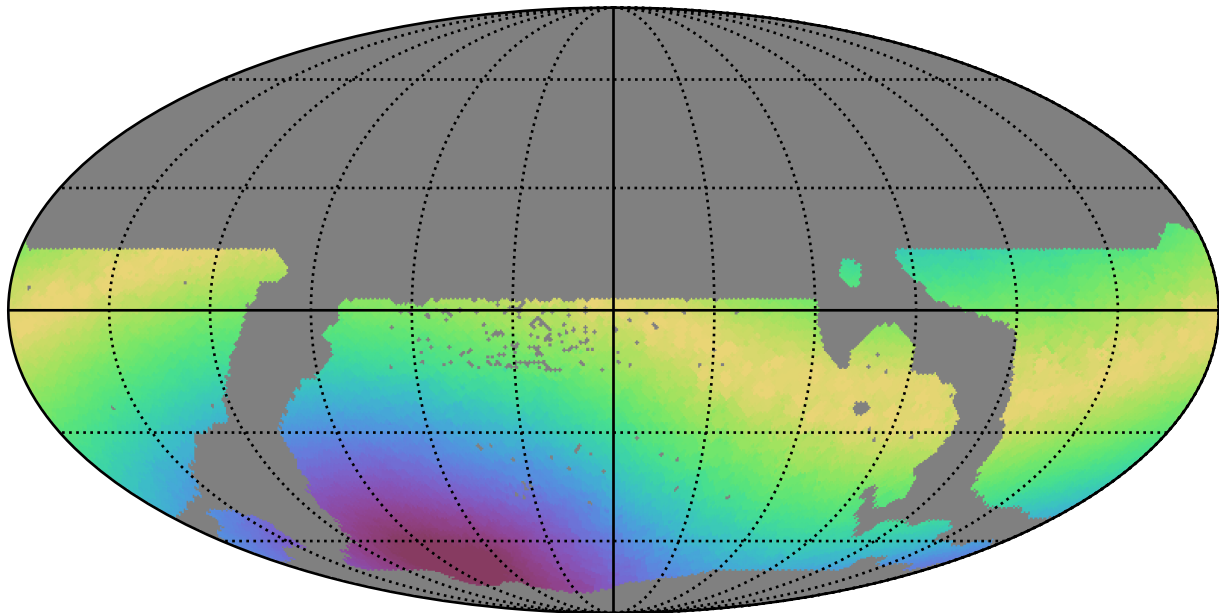
weather_cloudso30v3.4_10yrs WFD r band: Max moonDistance
