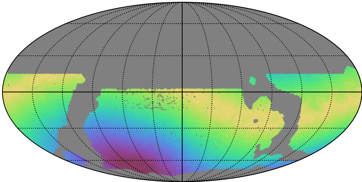
weather_cloudso30v3.4_10yrs WFD i band: Max moonDistance
