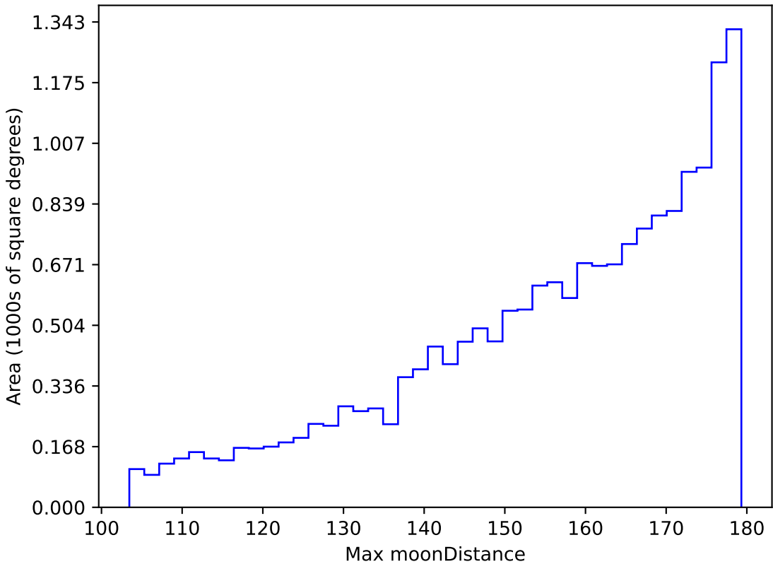
weather_cloudso30v3.4_10yrs WFD i band: Max moonDistance
