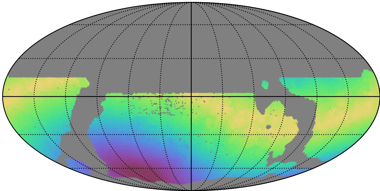
weather_cloudso30v3.4_10yrs WFD g band: Max moonDistance
