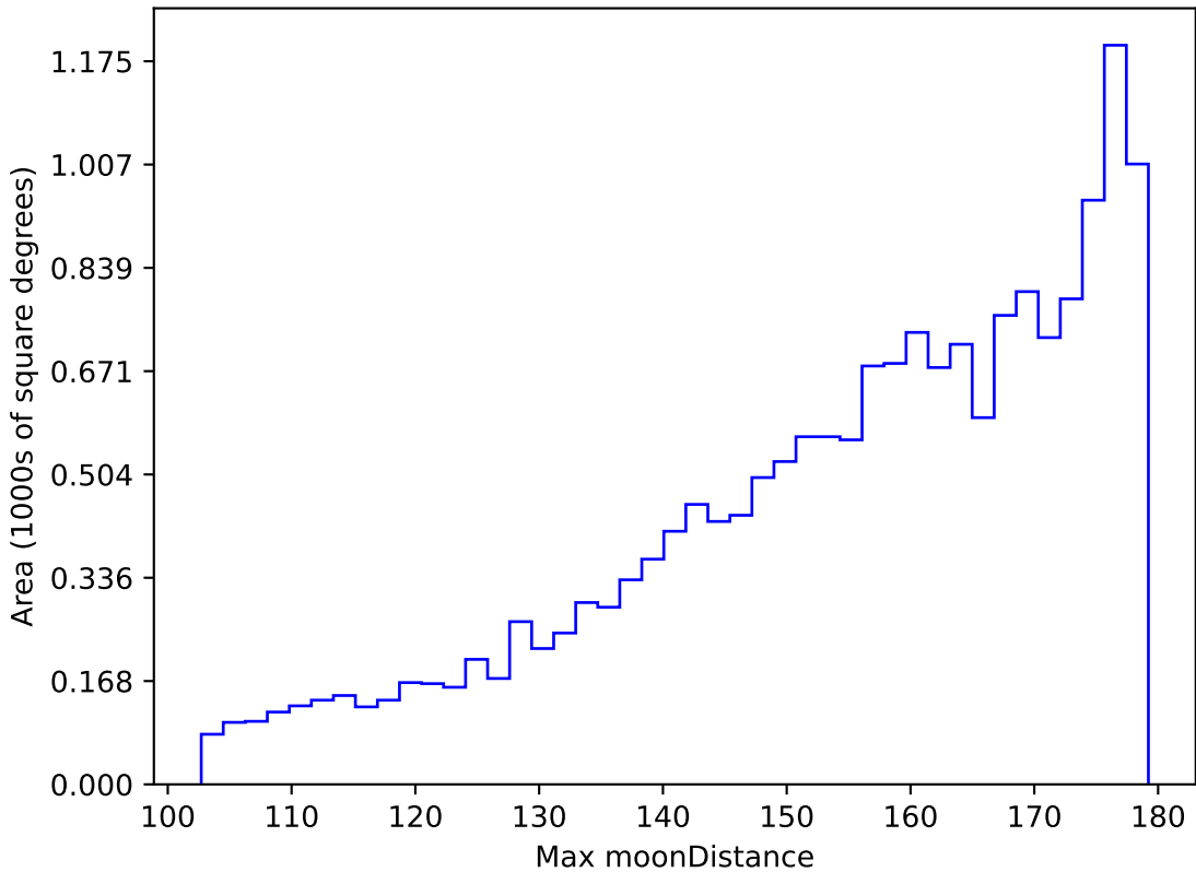
weather_cloudso30v3.4_10yrs WFD g band: Max moonDistance
