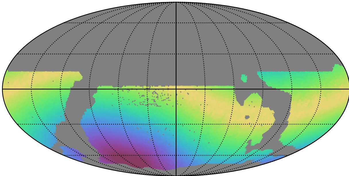
weather_cloudso30v3.4_10yrs WFD all bands: Max moonDistance
