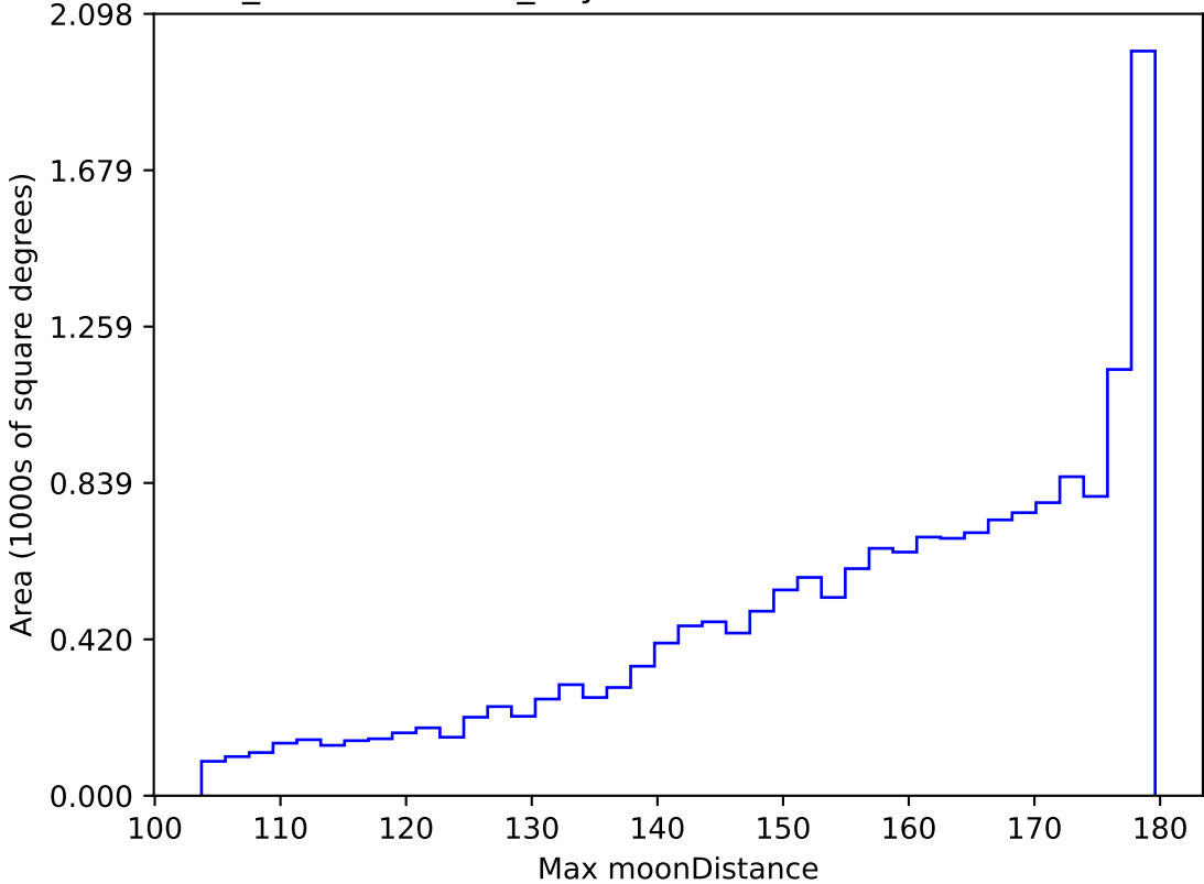
weather_cloudso30v3.4_10yrs WFD all bands: Max moonDistance
