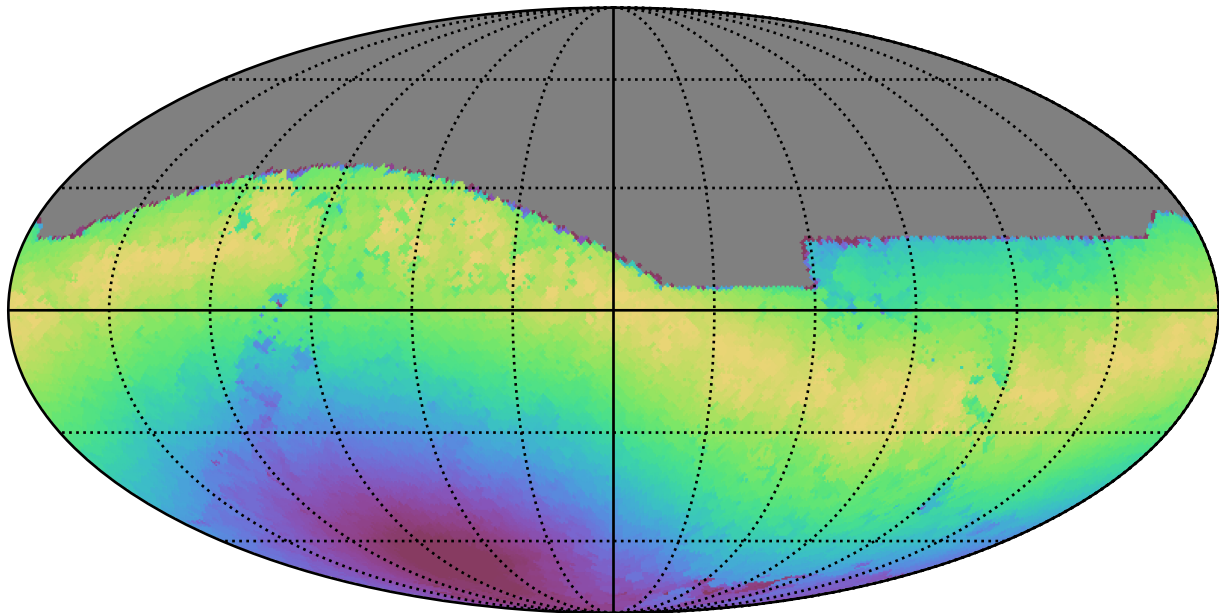
weather_cloudso30v3.4_10yrs All sky z band: Max moonDistance
