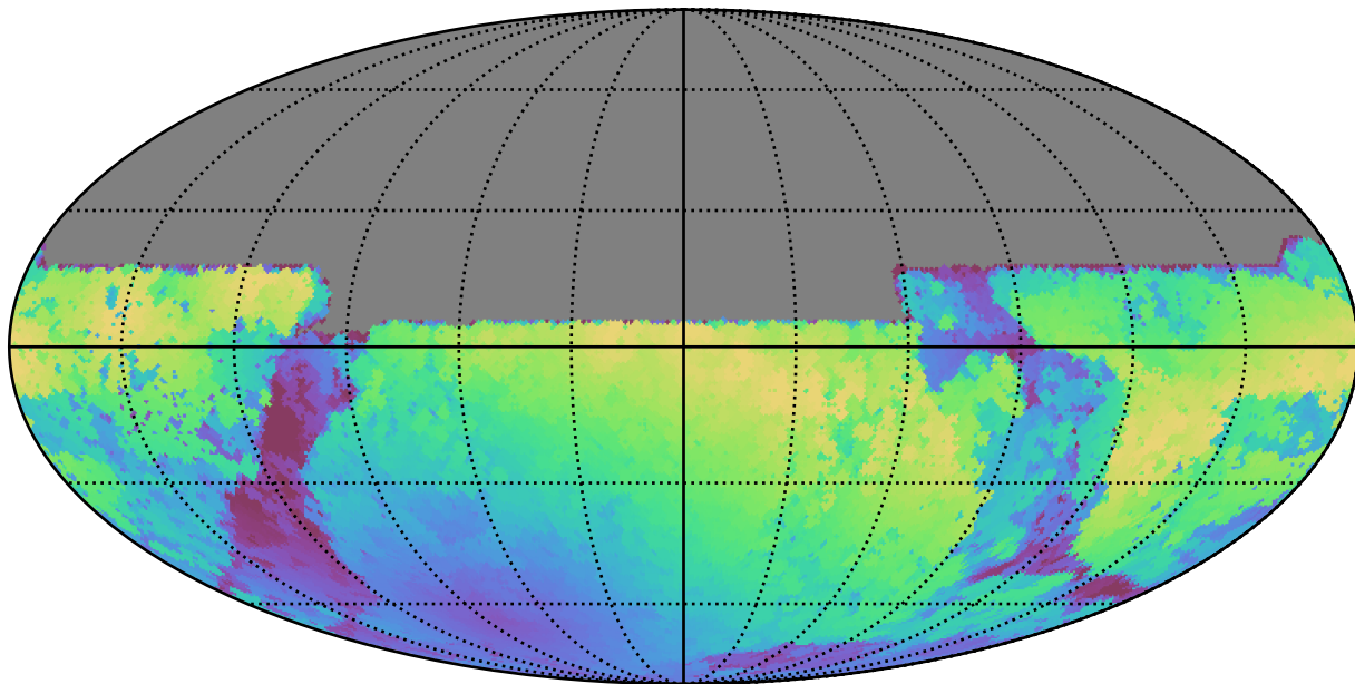
weather_cloudso30v3.4_10yrs All sky y band: Max moonDistance
