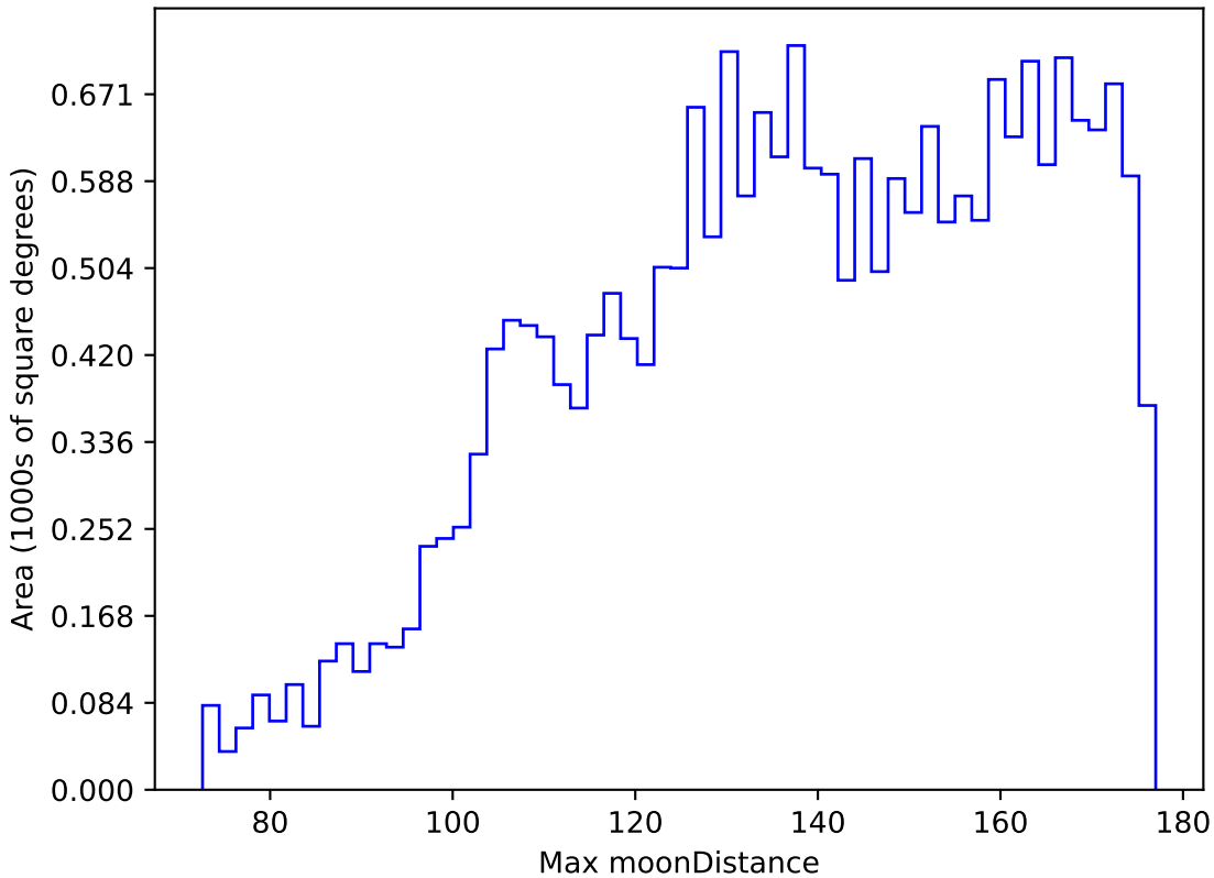
weather_cloudso30v3.4_10yrs All sky y band: Max moonDistance
