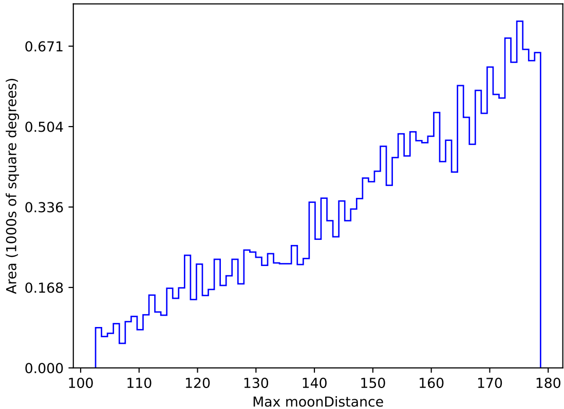
weather_cloudso30v3.4_10yrs All sky u band: Max moonDistance
