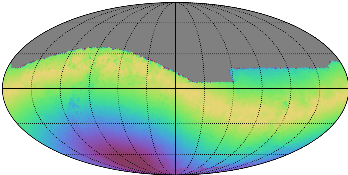
weather_cloudso30v3.4_10yrs All sky i band: Max moonDistance
