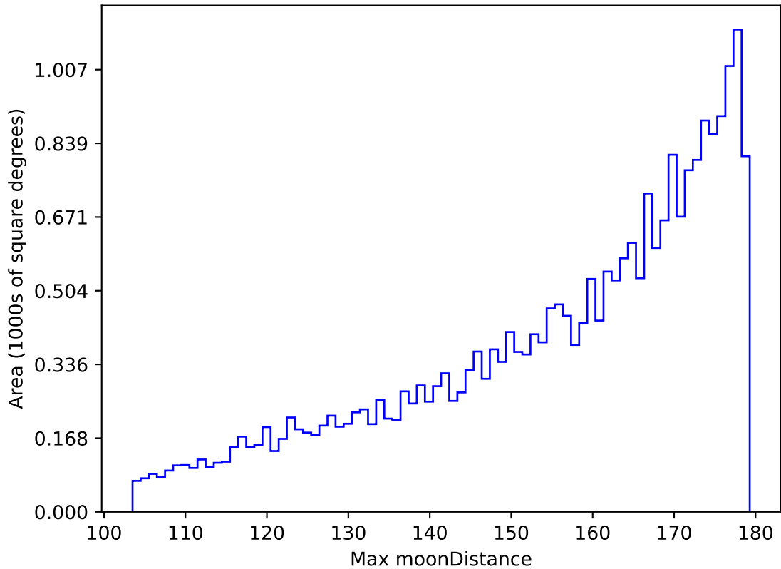
weather_cloudso30v3.4_10yrs All sky i band: Max moonDistance
