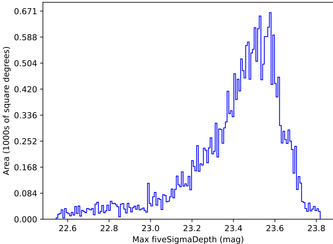
weather_cloudso30v3.4_10yrs Yr 1 z band: Max fiveSigmaDepth
