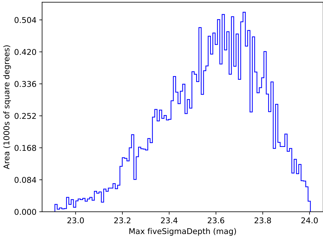
weather_cloudso30v3.4_10yrs Yr 1 u band: Max fiveSigmaDepth
