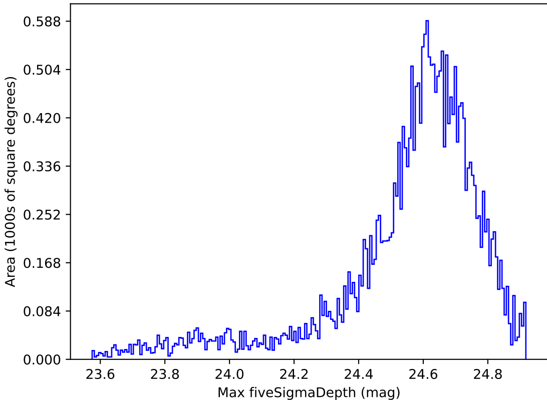
weather_cloudso30v3.4_10yrs Yr 1 r band: Max fiveSigmaDepth
