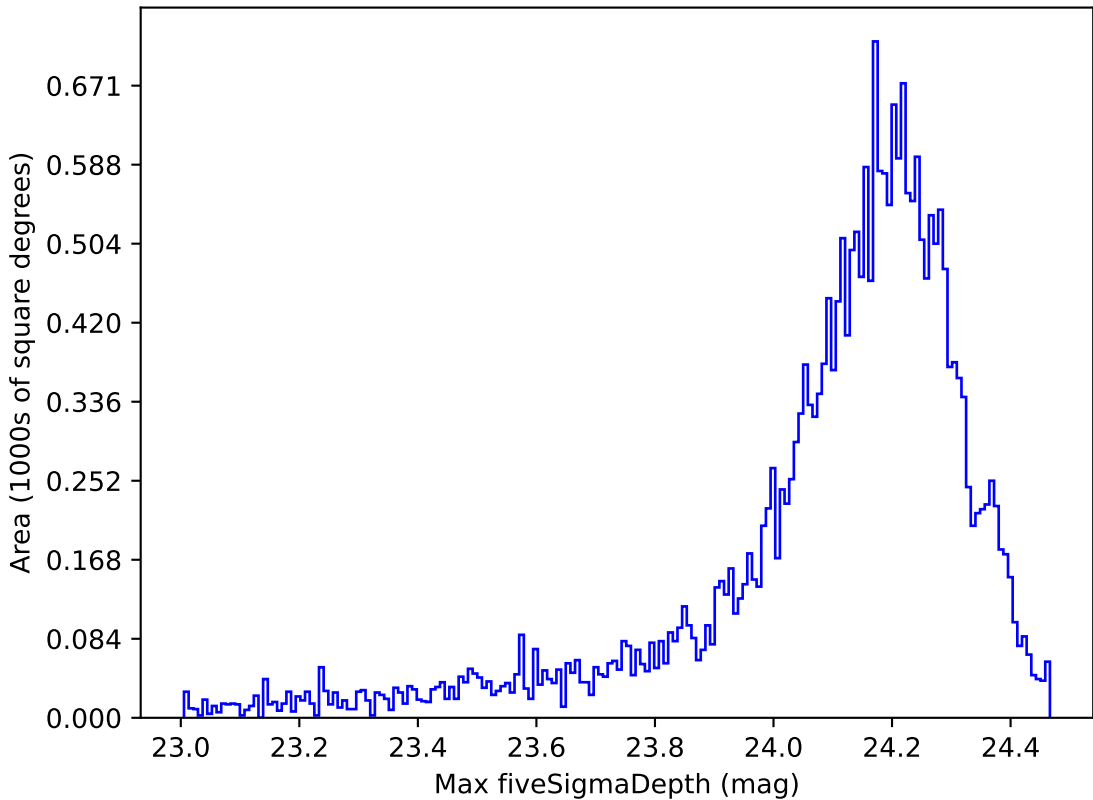
weather_cloudso30v3.4_10yrs Yr 1 i band: Max fiveSigmaDepth
