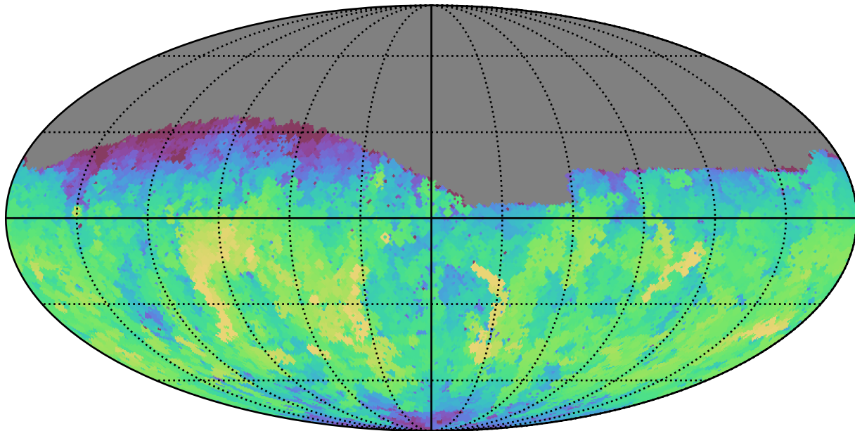
weather_cloudso30v3.4_10yrs Yr 1 g band: Max fiveSigmaDepth
