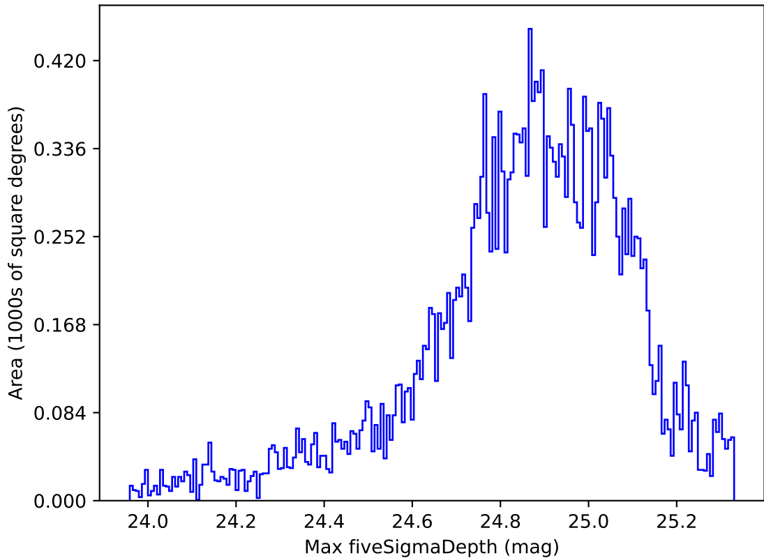
weather_cloudso30v3.4_10yrs Yr 1 g band: Max fiveSigmaDepth
