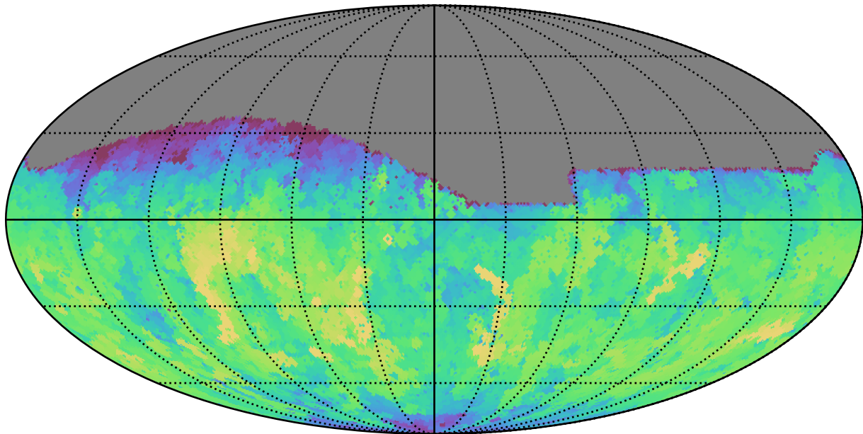
weather_cloudso30v3.4_10yrs Yr 1 all bands: Max fiveSigmaDepth
