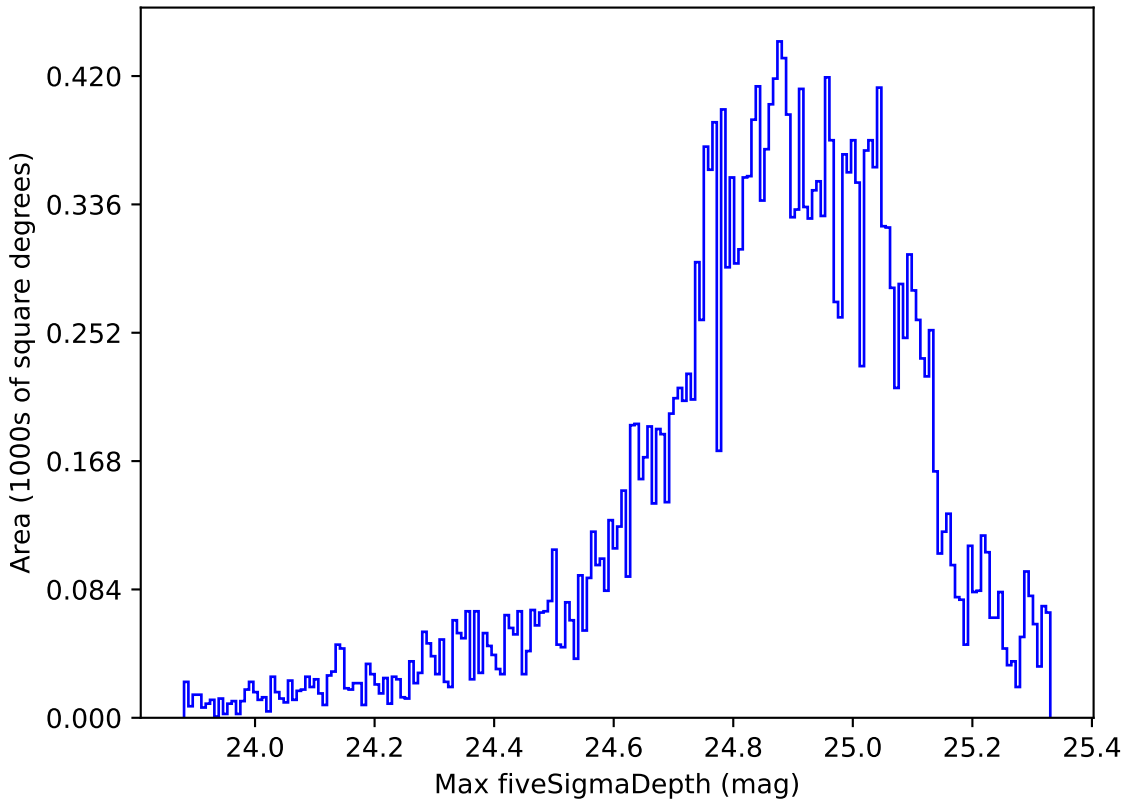
weather_cloudso30v3.4_10yrs Yr 1 all bands: Max fiveSigmaDepth
