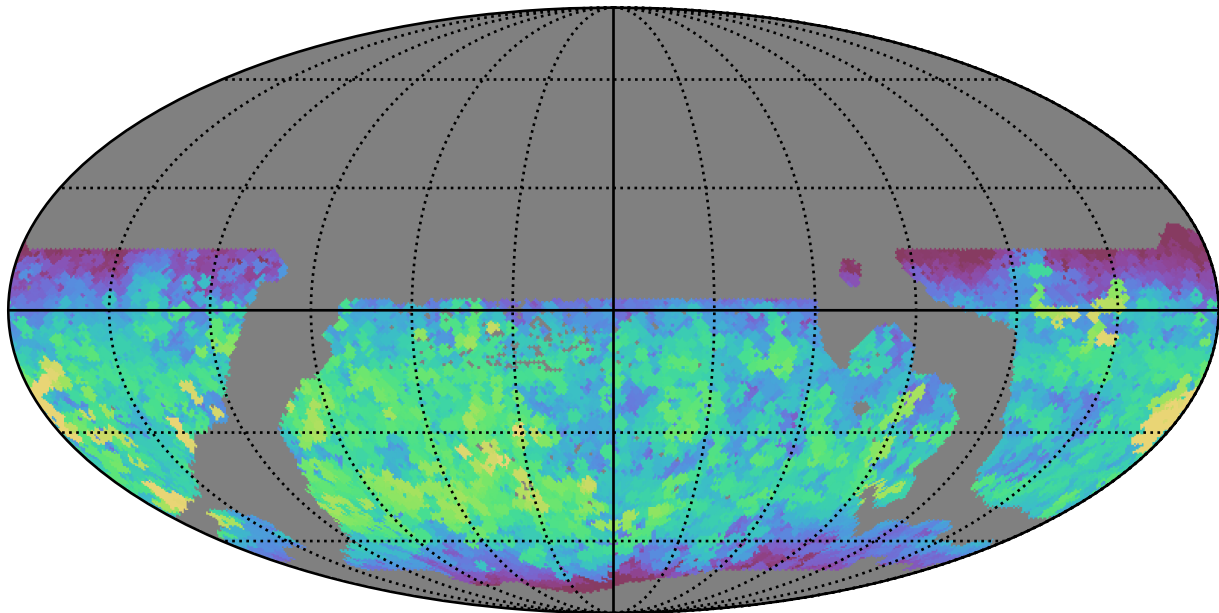
weather_cloudso30v3.4_10yrs WFD z band: Max fiveSigmaDepth
