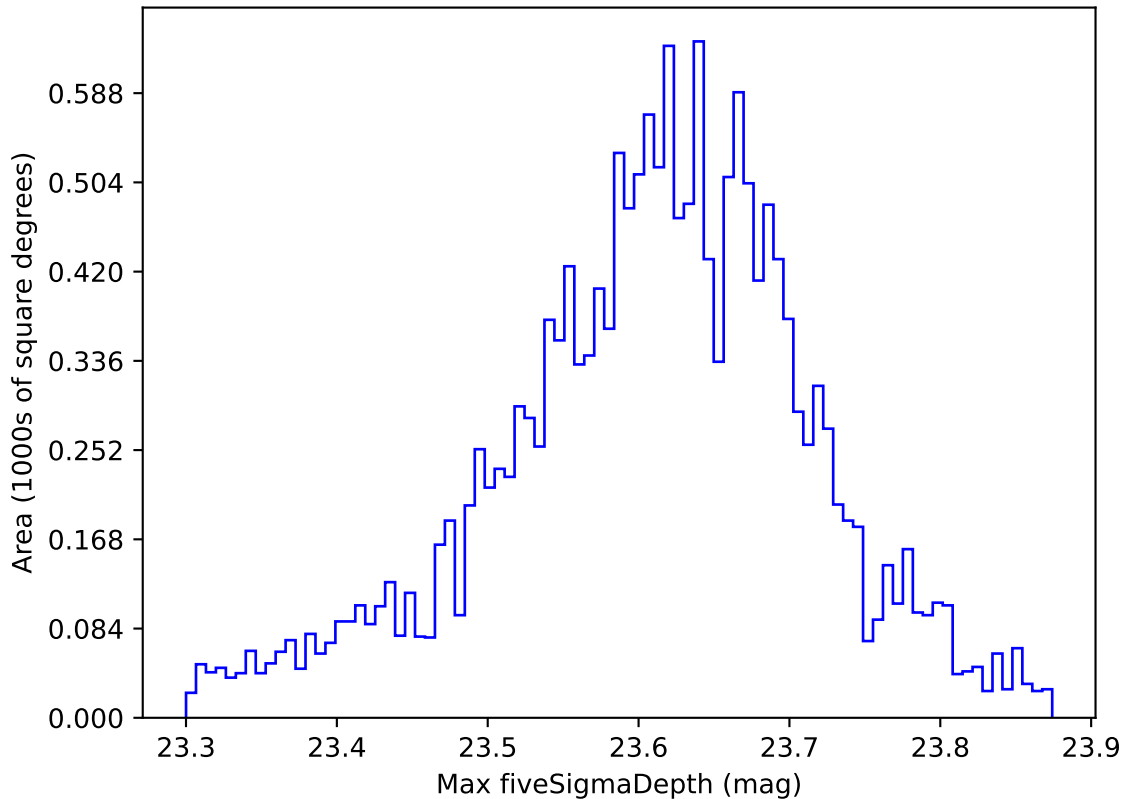
weather_cloudso30v3.4_10yrs WFD z band: Max fiveSigmaDepth
