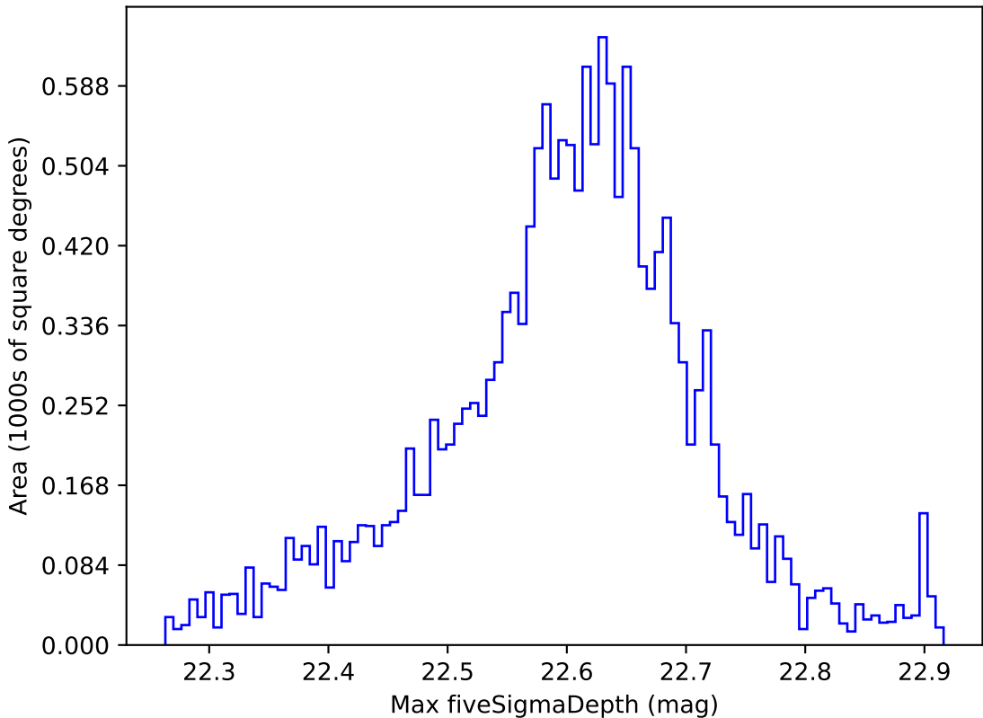
weather_cloudso30v3.4_10yrs WFD y band: Max fiveSigmaDepth
