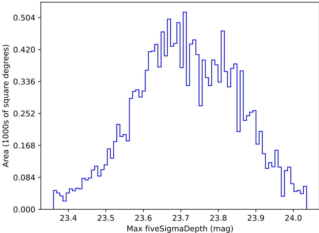
weather_cloudso30v3.4_10yrs WFD u band: Max fiveSigmaDepth
