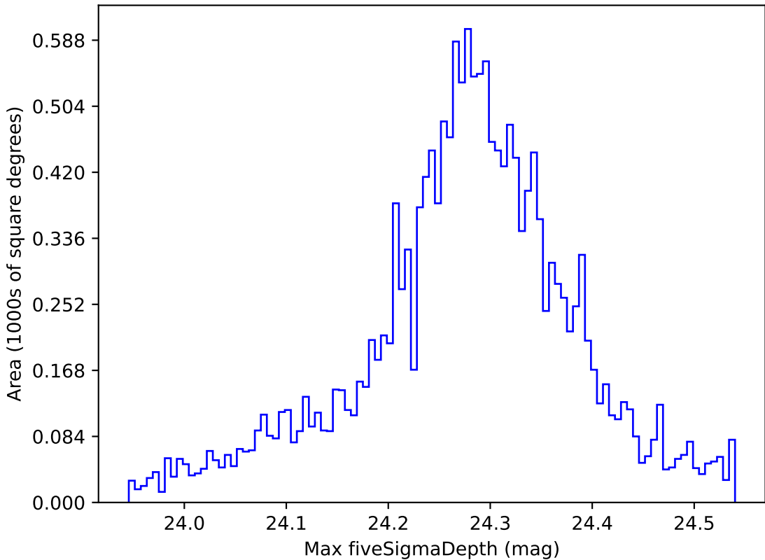
weather_cloudso30v3.4_10yrs WFD i band: Max fiveSigmaDepth
