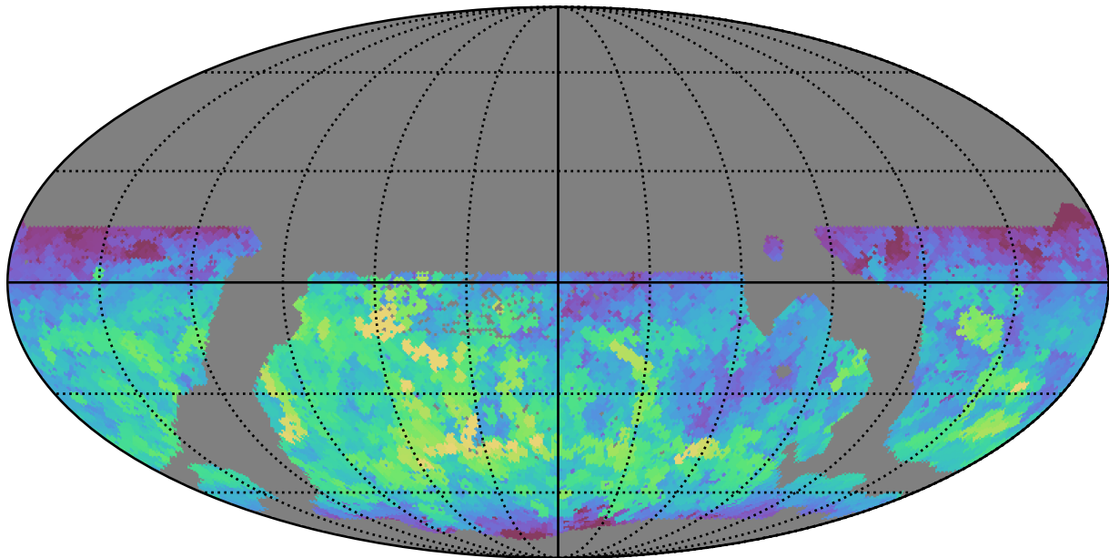
weather_cloudso30v3.4_10yrs WFD g band: Max fiveSigmaDepth
