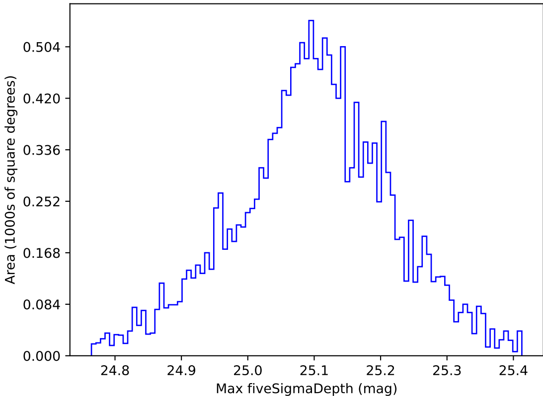
weather_cloudso30v3.4_10yrs WFD g band: Max fiveSigmaDepth
