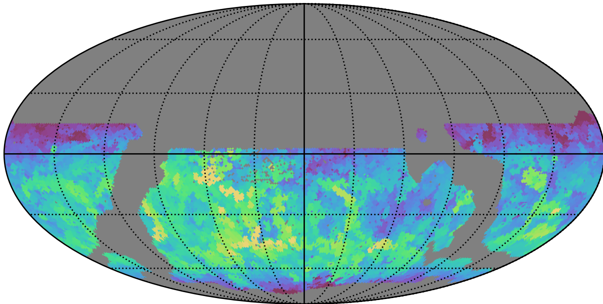
weather_cloudso30v3.4_10yrs WFD all bands: Max fiveSigmaDepth
